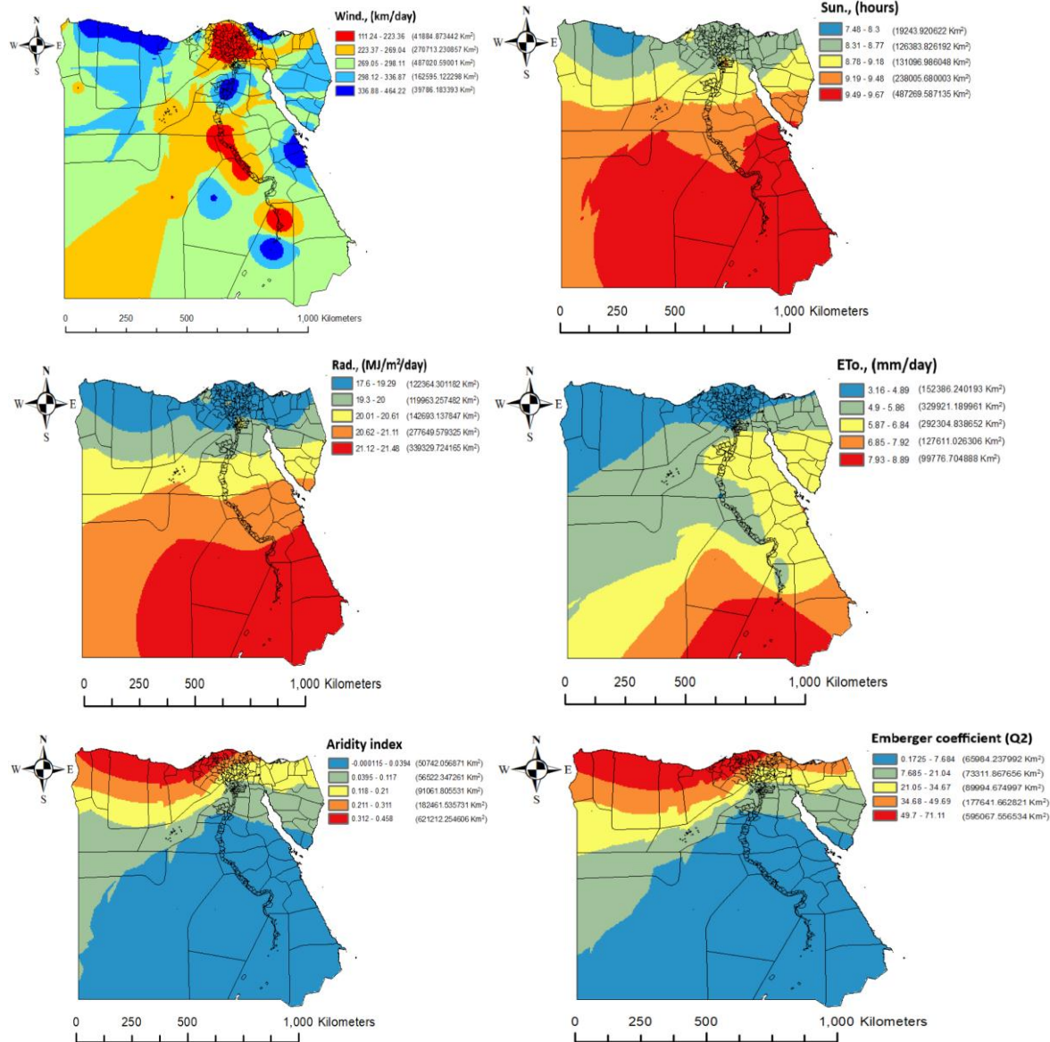
Fig. 5. Spatial distribution map of [The Wind speed (km/day), The Sunshine period (hr), The Radiation (MJ/m²/day), The Aridity Index (AI) and (ETo) the reference evapotranspiration in millimeters per day. Emberger's coefficient (Q2)] in Egypt from (1991-2020)
